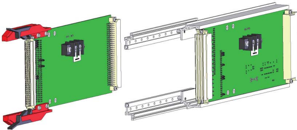
Figure 3-24: EC-96D1 and EC-48RD Direct Connect Extender Cards
