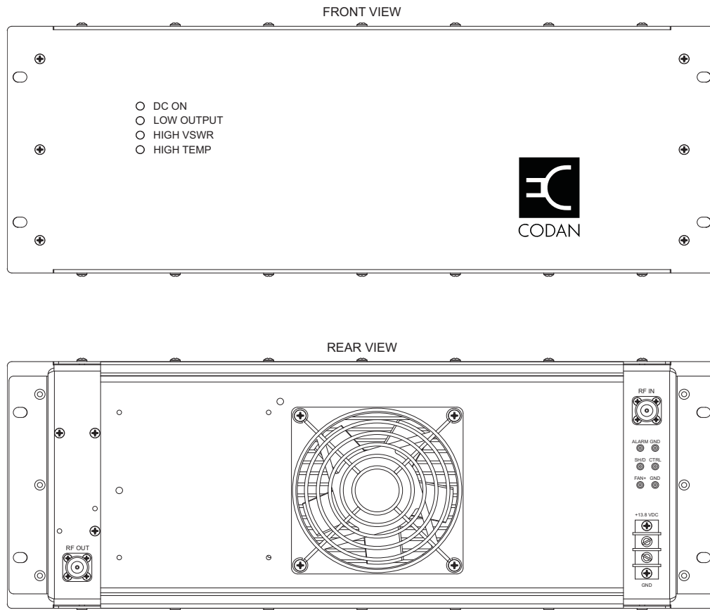
Figure 3-23: 100 Watt Power Amplifier
