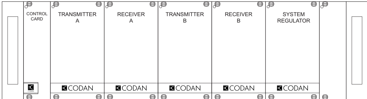
Figure 3-14: Standard Subrack Configuration
