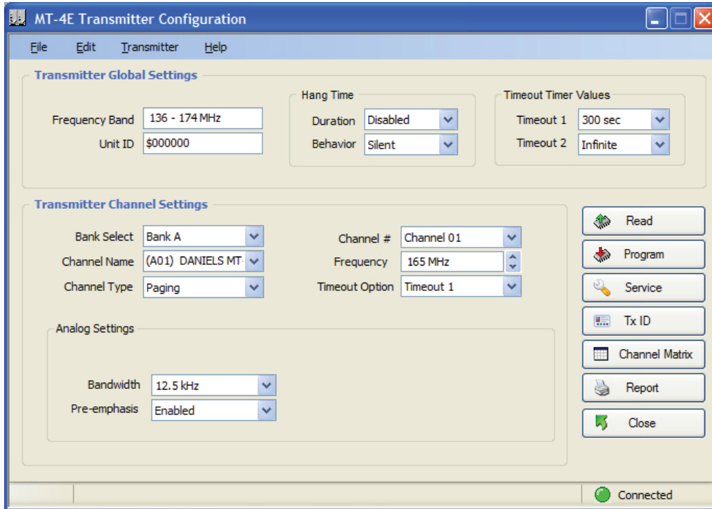
Figure 4-2: MT-4E Transmitter Program Example
