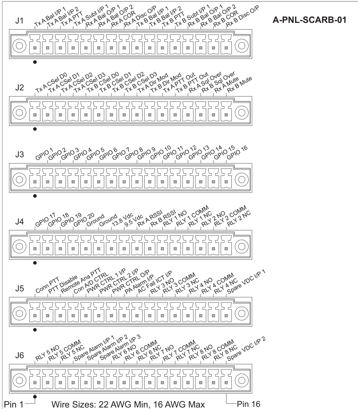
Figure 3-21: System Control and Relay Board Pin-Out
